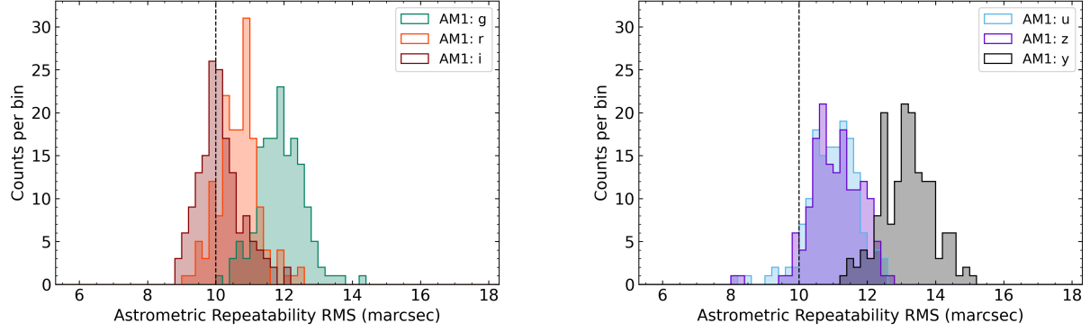
Figure 7: The distributions of the RMS values of the astrometric repeatability on 5' timescales in the a) g , r , and i ) and b) u , z , and y bands of sources detected as part of the DP0.2 processing campaign. The vertical dashed lines show the LSST SRD design specifications.
