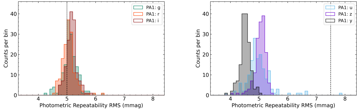
Figure 8: The distributions of the RMS values of the photometric repeatability of bright non-saturated unresolved point sources in the a) g , r , and i ) and b) u , z , and l ) bands of sources detected as part of the DP0.2 processing campaign. The vertical dashed lines show the LSST SRD design specifications.
