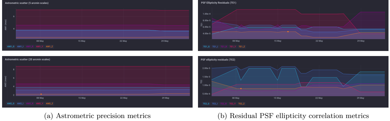
Figure 4: Examples of the time evolution of four faro metrics computed on a nightly cadence in CI over a period of one month on the outputs of the nightly data release processing of a small subset of the HSC PDR2 dataset. Left shows the AM1 metric that characterizes the astrometric scatter on two different spatial scales, 5 and 20 arcmins, and right shows the residual PSF ellipticity correlations, TE1 and TE2.
